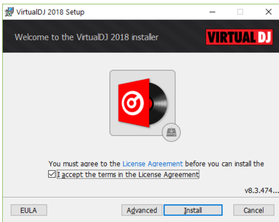
Fig. 1: VirtualDJ | Installation
