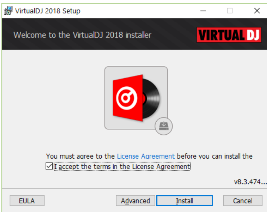
Abb. 1: VirtualDJ | Installation
